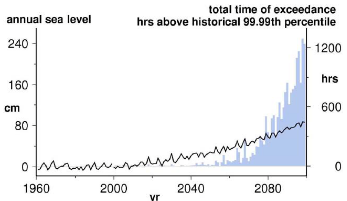
Figure 5-5: Projected number of hours (blue bars) of extremely high sea level off San Francisco under an assumed sea-level rise and climate change scenario. In this exercise, a sea-level event registers as an exceedance when San Francisco’s projected sea level exceeds its recent (1970–2000) 99.99th percentile level, 1.41 meters (55 inches) above historical mean sea level. In the recent historical period, sea level has exceeded this threshold about one time (1 hour) every 14 months. Sea-level rise (black line) during 1960–1999 was arbitrarily set to zero, then increased to the committee’s projected level for the San Francisco area over the 21st century (92 cm). Source: Adapted from Cloern et al. (2011).
